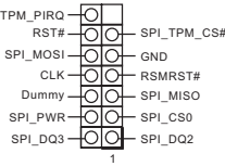
SPI_TPM_J1
